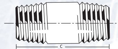
BARREL NIPPLE - TAPER THREAD
