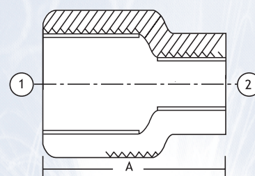
REDUCING SOCKET
